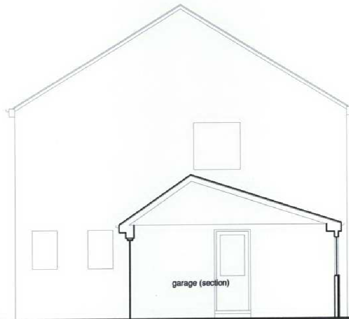
Gable Elevation - North ( existing )
